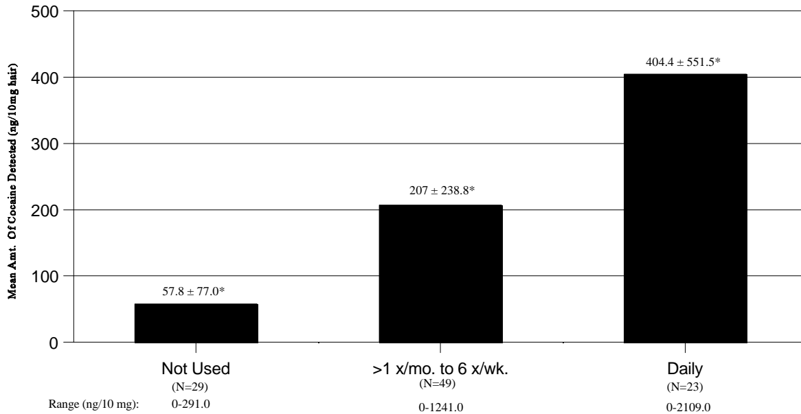
FIGURE 2 Amount of Cocaine Detected in Hair at Intake, by Self-Reported Use in the Past 30 Days (N=101 clients)
