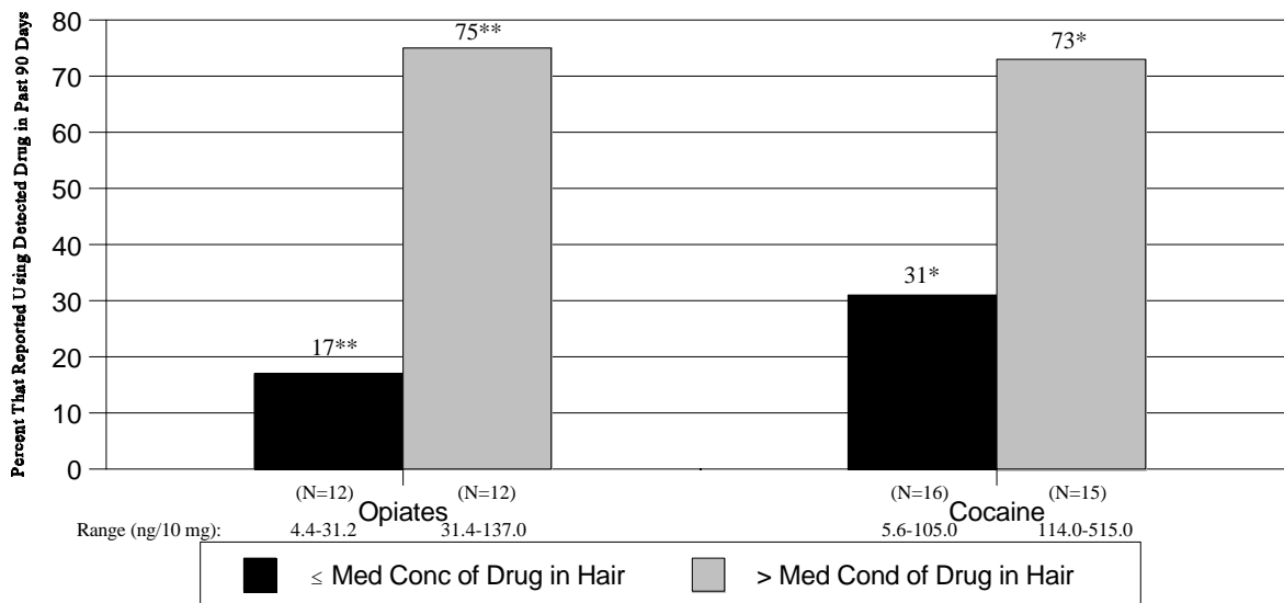
FIGURE 3 Percentage of Persons Testing Positive for Opiates or Cocaine at Follow-up Who Reported Using the Detected Drug in the Past 90 Days, by Amount of Drug Detected in Hair
