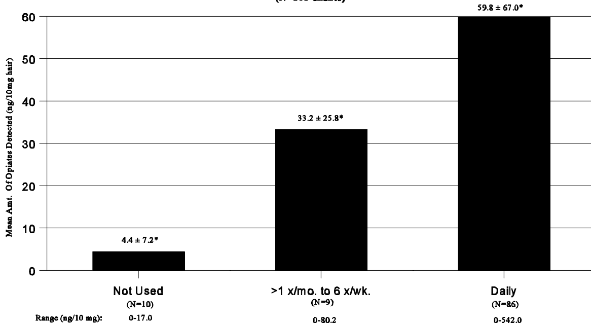
FIGURE 1 Amount of Opiates Detected in Hair at Intake, by Self-Reported Use in the Past 30 Days (N=105 clients)
